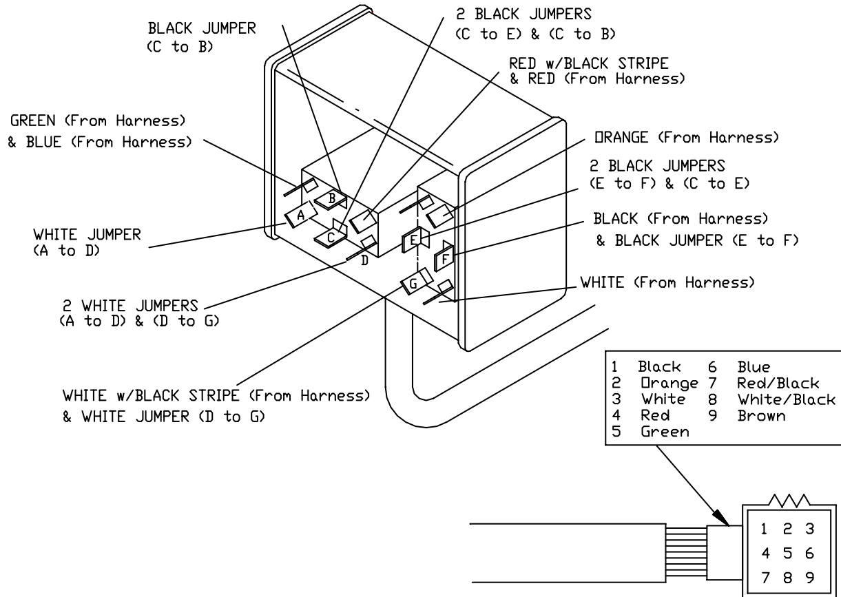
Figure 1. Straight Blade Rocker Box Wiring Diagram
