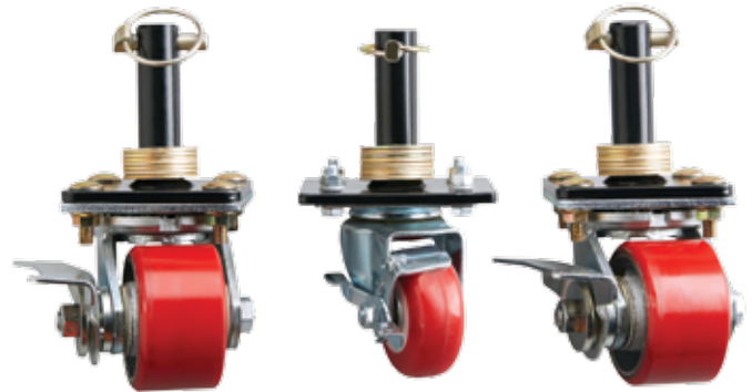
V-Blade Dolly Wheel Kit
